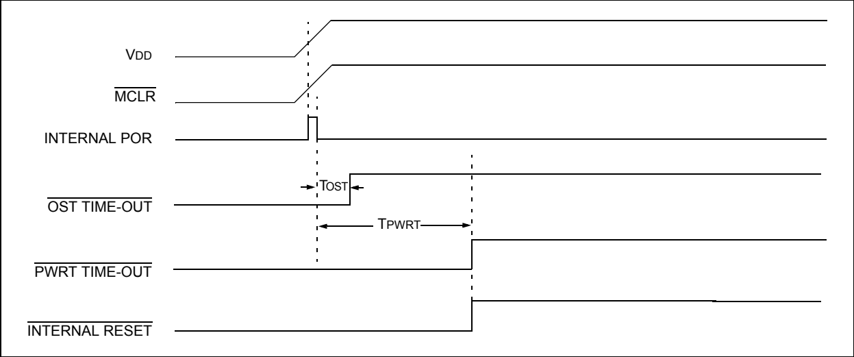
FIGURE 21-3: TIME-OUT SEQUENCE ON POWER-UP ( \overline{\text{MCLR}} TIED TO \text{V}_{\text{DD}} )
