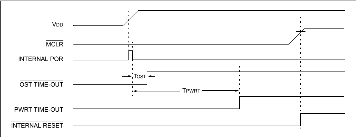
FIGURE 21-5: TIME-OUT SEQUENCE ON POWER-UP ( \overline{\text{MCLR}} NOT TIED TO \text{V}_{\text{DD}} ): CASE 2
