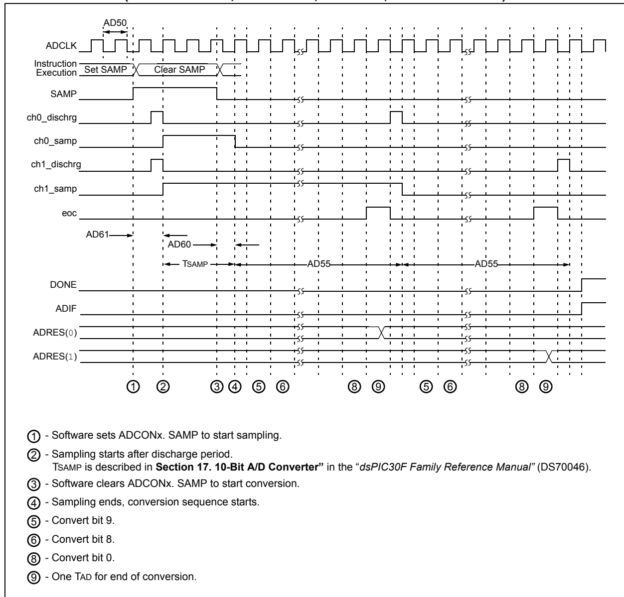
FIGURE 24-25: 10-BIT HIGH-SPEED A/D CONVERSION TIMING CHARACTERISTICS (CHPS<1:0> = 01, SIMSAM = 0, ASAM = 0, SSR<2:0> = 000)
