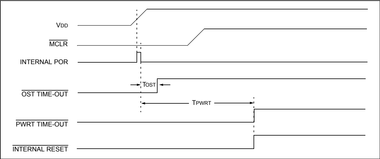
FIGURE 21-4: TIME-OUT SEQUENCE ON POWER-UP ( \overline{\text{MCLR}} NOT TIED TO \text{V}_{\text{DD}} ): CASE 1
