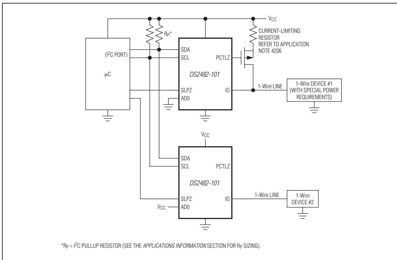
Figure 10. Application Schematic
