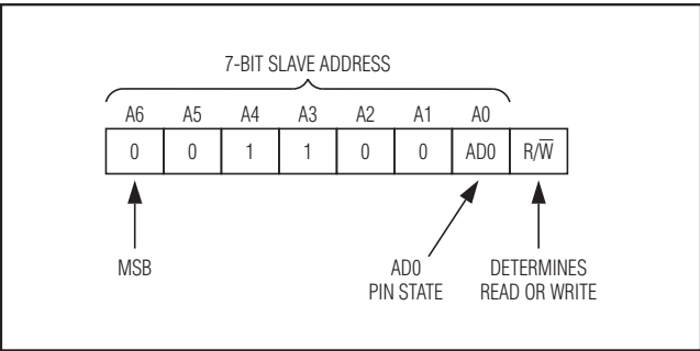
Figure 8. DS2482-101 Slave Address
