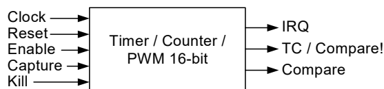
Figure 7-15. Timer/Counter/PWM
