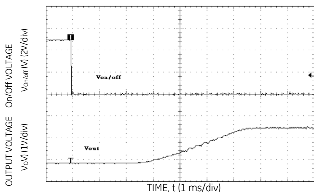
Figure 15. Typical Start-Up Using Remote On/Off with Low-ESR external capacitors (7x150µF Polymer) ( V_{in} = 12 Vdc, V_o = 3.3 Vdc, I_o = 5.0 A, C_o = 1050 µF).
