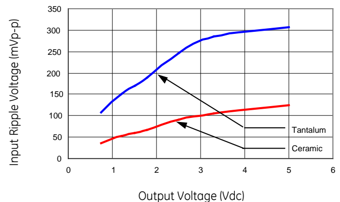
Figure 26. Input ripple voltage for various output with 2x47 μF tantalum capacitors and with 2x22 μF ceramic capacitors at the input (100% of I_{O,max} ).
