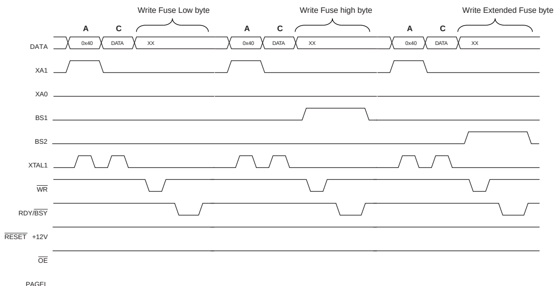
Figure 21-5. Fuses Programming Waveforms
