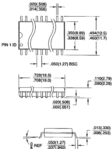
28R, 28 Lead, 0.330" Wide, Plastic Gull Wing Small Outline (SOIC) JEDEC STANDARD MS-012 AC
