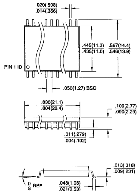
32R, 32 Lead, 0.440" Wide, Plastic Gull Wing Small Outline (SOIC) JEDEC STANDARD MS-012 AC
