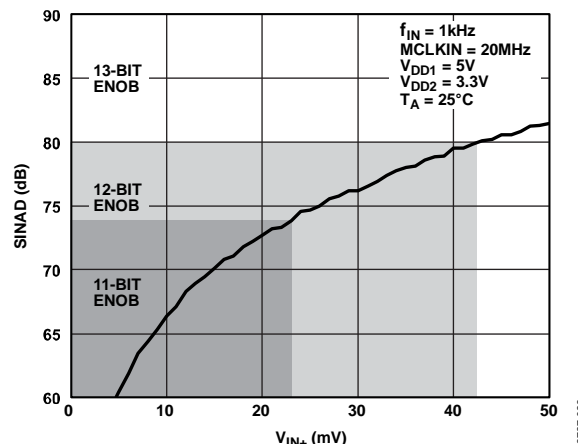
Figure 28. SINAD vs. V_{IN+} AC Input Signal Amplitude
