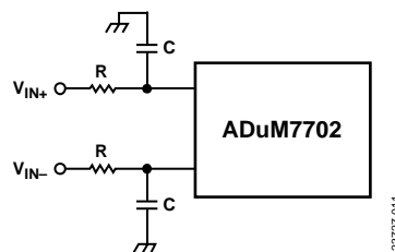
Figure 29. RC Low-Pass Filter Input Network
