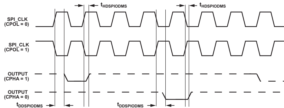
Figure 35. ODM Slave
