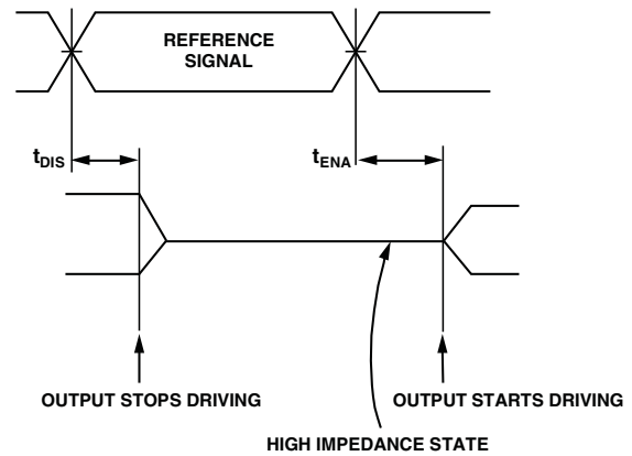
Figure 62. Output Enable/Disable
