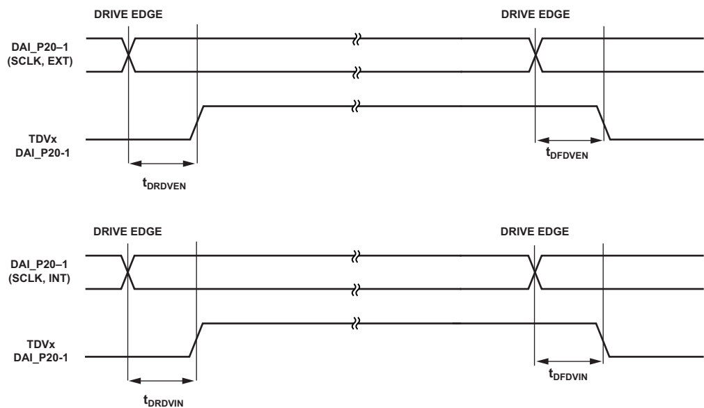
Figure 23. Serial Ports—TDM Internal and External Clock
