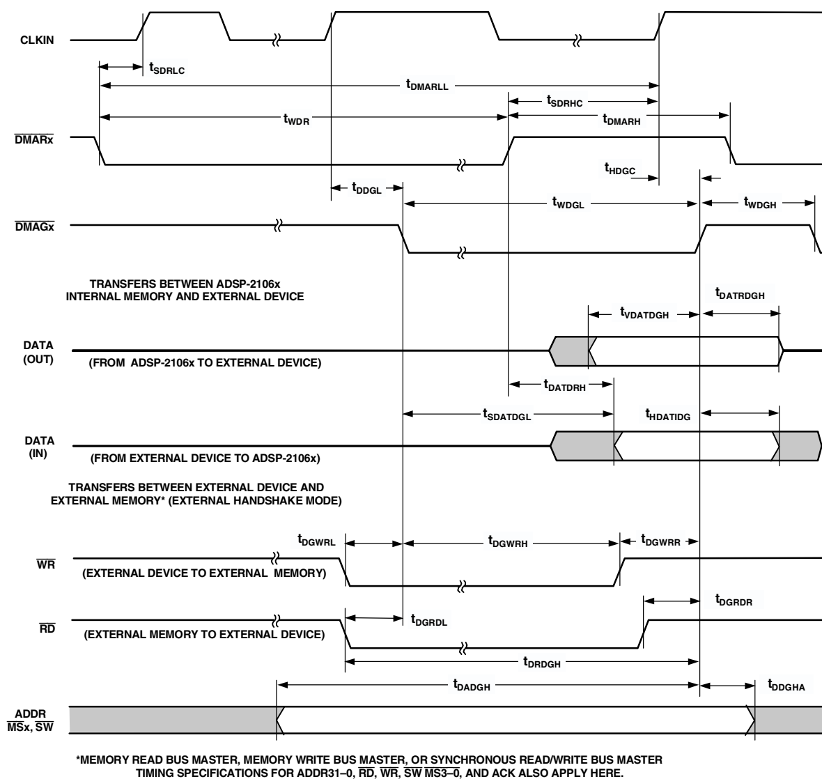
Figure 23. DMA Handshake
