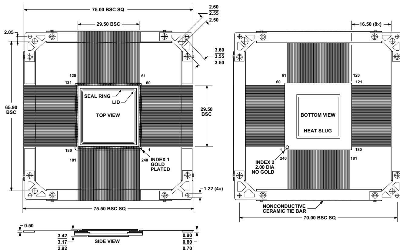
Figure 45. 240-Lead Ceramic Quad Flat Package, Mounted with Cavity Up [CQFP] (OS-240-1B)
