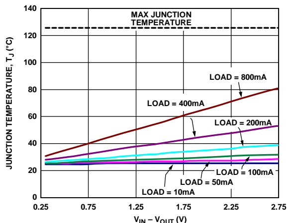
Figure 44. 1000 mm² of PCB Copper, T_B = 25^\circ\text{C} , LFCSP
