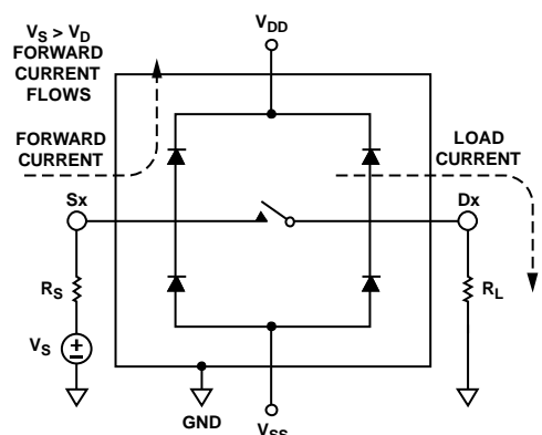
Figure 33. ESD Protection Diodes on Conventional CMOS Switch
