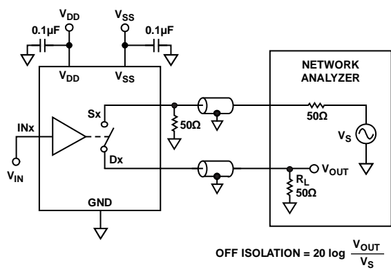
Figure 28. Off Isolation
