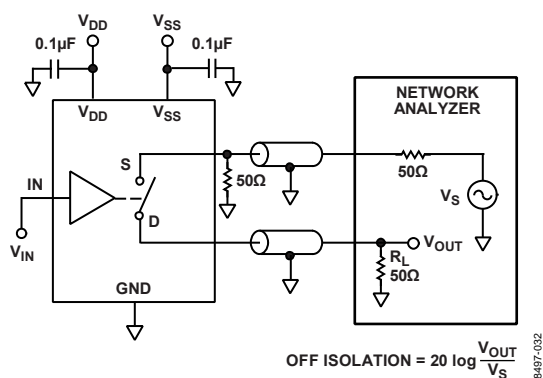
Figure 26. Off Isolation
