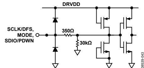
Figure 32. Equivalent SCLK/DFS, MODE and SDIO/PDWN Input Circuit
