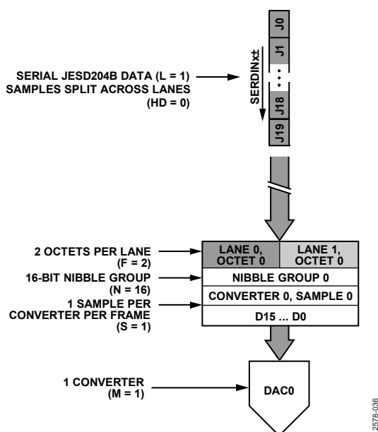
Figure 64. JESD204B Mode 10 Data Deframing
