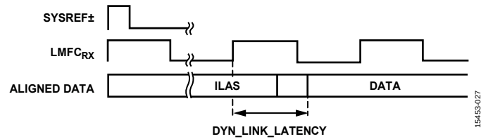
Figure 61. DYN_LINK_LATENCY_x Illustration
