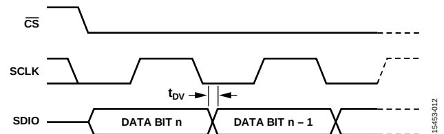
Figure 44. Timing Diagram for Serial Port Register Read
