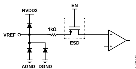
Figure 86. VREF
