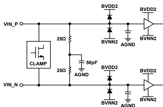
Figure 77. Analog Inputs
