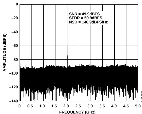
Figure 41. Single-Tone FFT with f_{IN} = 4 GHz, 10 GSPS
