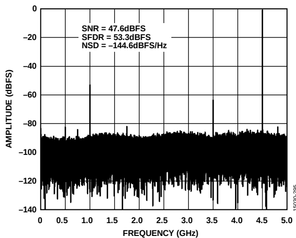
Figure 42. Single-Tone FFT with f_{IN} = 5.5 GHz, 10 GSPS
