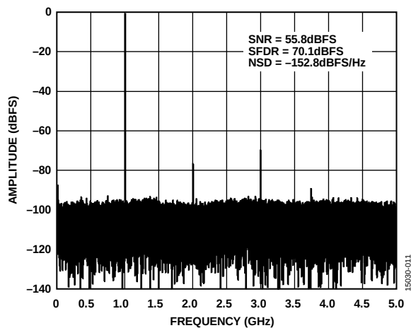
Figure 39. Single-Tone FFT with f_{IN} = 1 GHz, 10 GSPS
