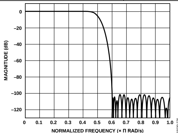
Figure 108. TB2 Filter Response
