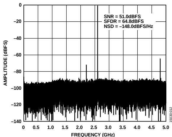
Figure 40. Single-Tone FFT with f_{IN} = 2.6 GHz, 10 GSPS
