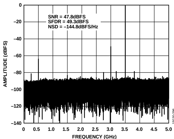
Figure 43. Single-Tone FFT with f_{IN} = 6.5 GHz, 10 GSPS
