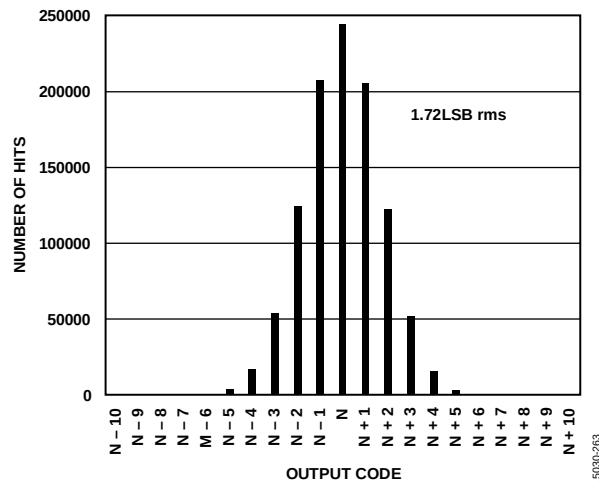
Figure 71. Input-Referred Noise Histogram, 10 GSPS
