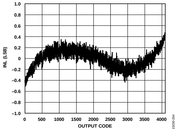
Figure 31. INL at f_{IN} = 170 MHz, 6 GSPS
