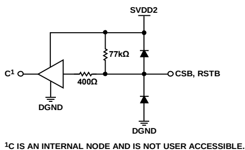
Figure 83. CSB and RSTB
