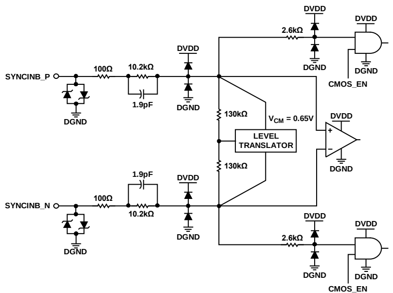
Figure 88. SYNCINB_x Inputs
