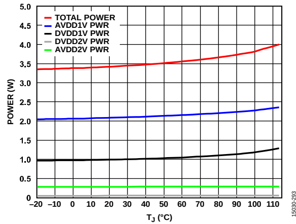
Figure 36. Power vs. Junction Temp ( T_J ), f_{IN} = 2600 MHz, 6 GSPS
