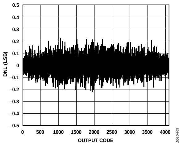
Figure 32. DNL at f_{IN} = 170 MHz, 6 GSPS
