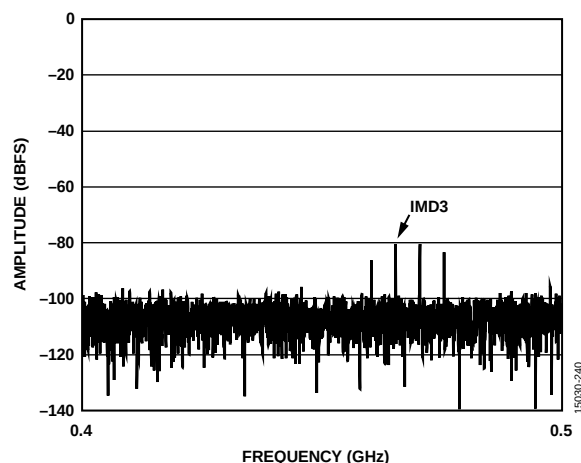
Figure 25. Two-Tone FFT, IMD3 Zoom In, f_{IN1} = 1841.5 MHz, f_{IN2} = 1846.5 MHz, A_{IN1} and A_{IN2} = -7 dBFS (see Figure 23), 6 GSPS
