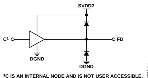
Figure 85. FD
