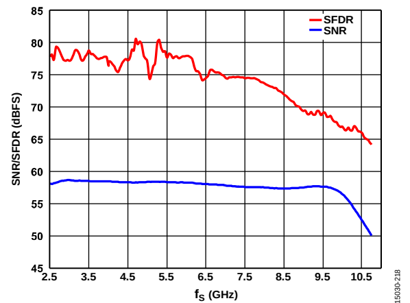
Figure 48. SNR/SFDR vs. Sampling Frequency, f_{IN} = 170 MHz
