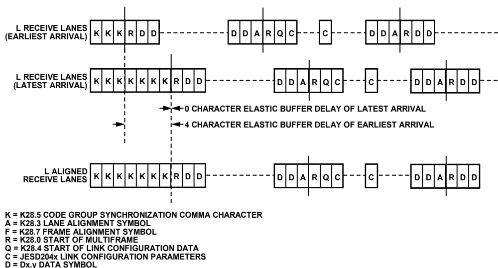
Figure 99. Lane Alignment During ILAS
