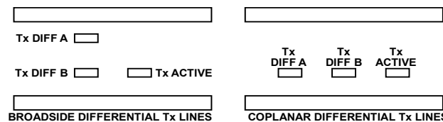
Figure 125. Broadside vs. Coplanar Differential Stripline Routing Techniques
