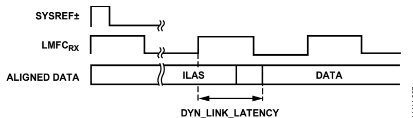
Figure 106. DYN_LINK_LATENCY_x Illustration
