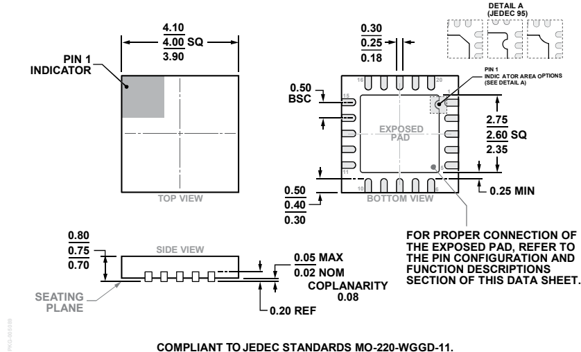
Figure 49. 20-Lead Lead Frame Chip Scale Package [LFCSP]
