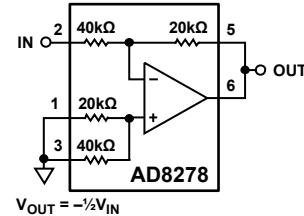
Figure 55. Inverting Amplifier, Gain = -1/2
