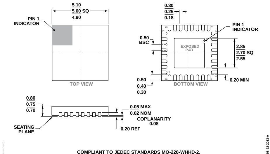
COMPLIANT TO JEDEC STANDARDS MO-220-WHHD-2. Figure 27. 32-Lead Lead Frame Chip Scale Package [LFCSP] 5 mm × 5 mm Body and 0.75 mm Package Height (CP-32-21) Dimensions shown in millimeters
