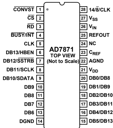
Figure 5. AD7871 PDIP
