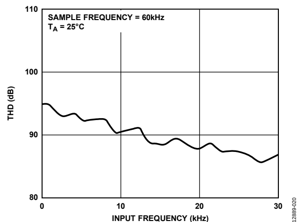
Figure 22. Total Harmonic Distortion vs. Frequency
