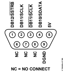
Figure 30. SKT5 Pinout
