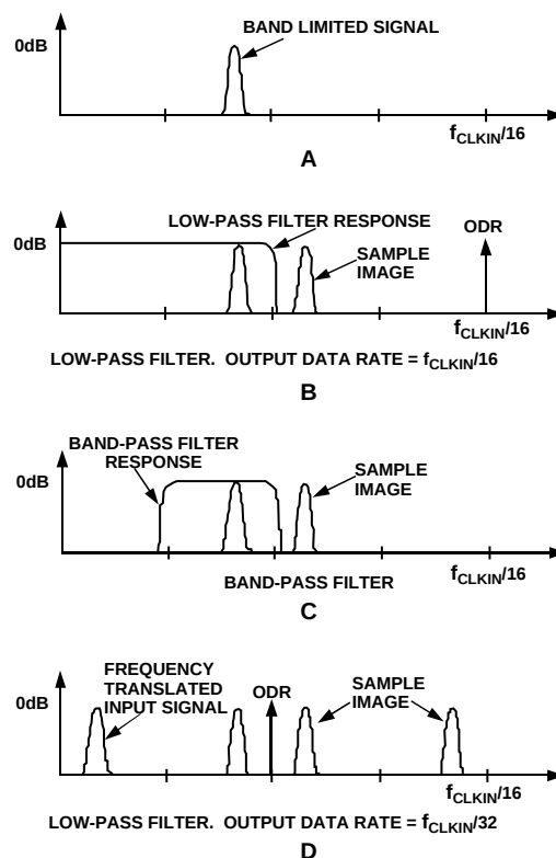
Figure 28. Band-Pass Operation
