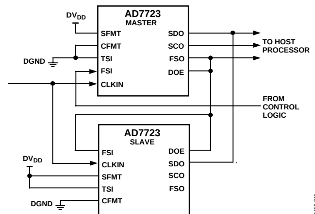
Figure 45. Serial Mode 1 Connection for Two-Channel Multiplexed Operation
