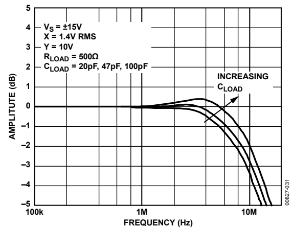
Figure 13. Gain vs. Frequency vs. C_{\text{LOAD}}
