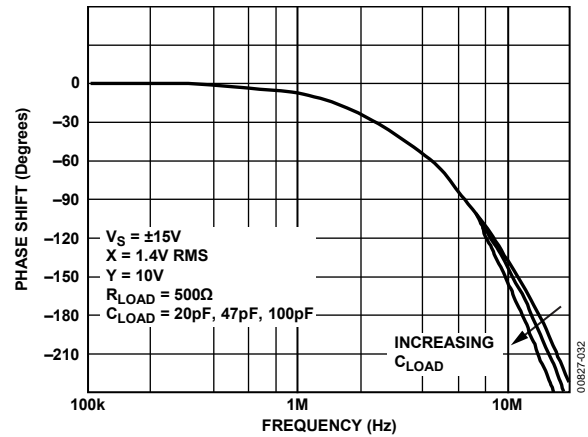
Figure 14. Phase vs. Frequency vs. C_{\text{LOAD}}
