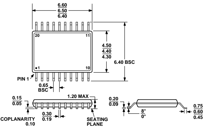
Figure 23. 20-Lead Thin Shrink Small Outline Package [TSSOP] (RU-20)
