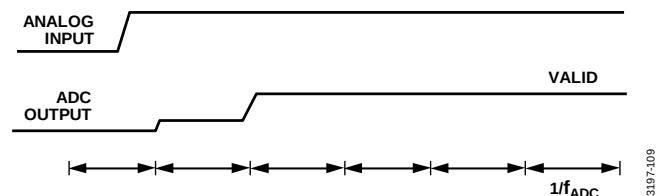
Figure 103. Step Change on the Analog Input, Sinc 4 + Sinc 1 Filter
