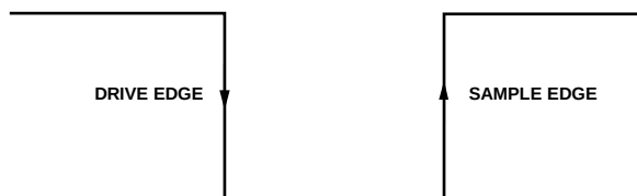
Figure 66. SPI Mode 3, SCLK Edges
