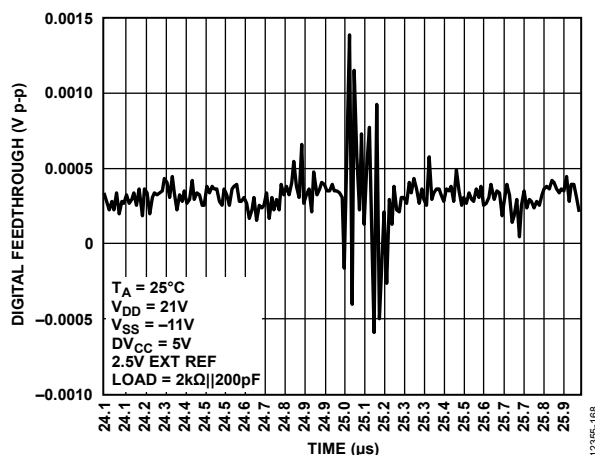
Figure 70. Digital Feedthrough
