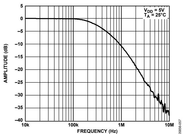
Figure 50. Multiplying Bandwidth
