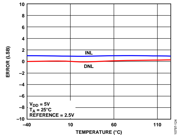
Figure 12. INL Error and DNL Error vs. Temperature
