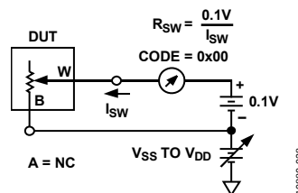
Figure 39. Incremental On Resistance
