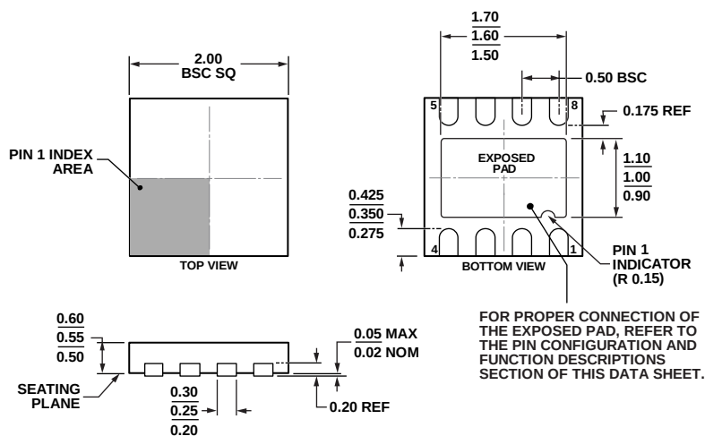
Figure 51. 8-Lead Frame Chip Scale Package[LFCSP_UD]
