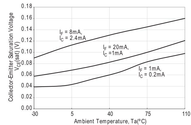
Figure 14 Collector-Emittter Saturation Voltage vs. Ambient Temperature
