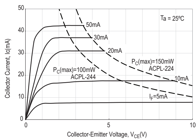
Figure 9 Collector Current vs. Collector-Emittter Voltage
