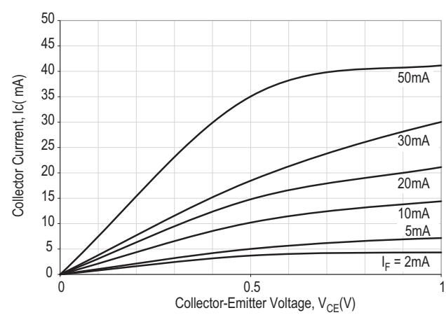
Figure 10 Collector Current vs. Small Collector-Emittter Voltage
