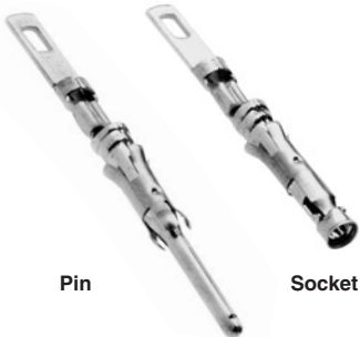
Solder-Tab
