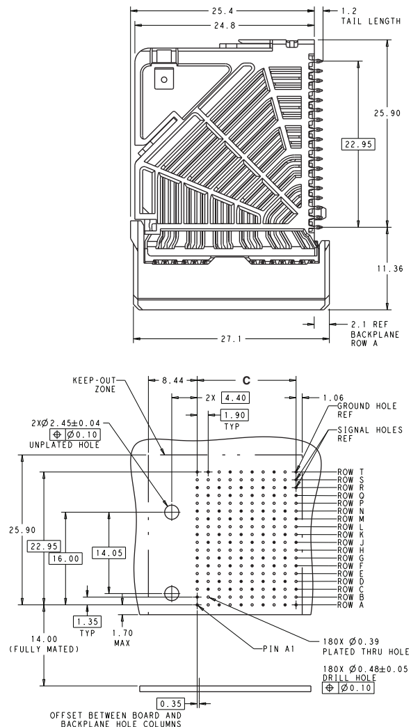
Recommended PCB Layout Min. Board Thickness 1.0
