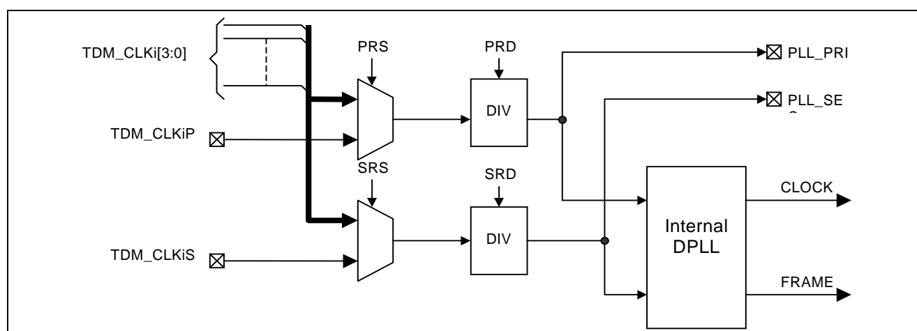
Figure 16 - Synchronous TDM Clock Generation
