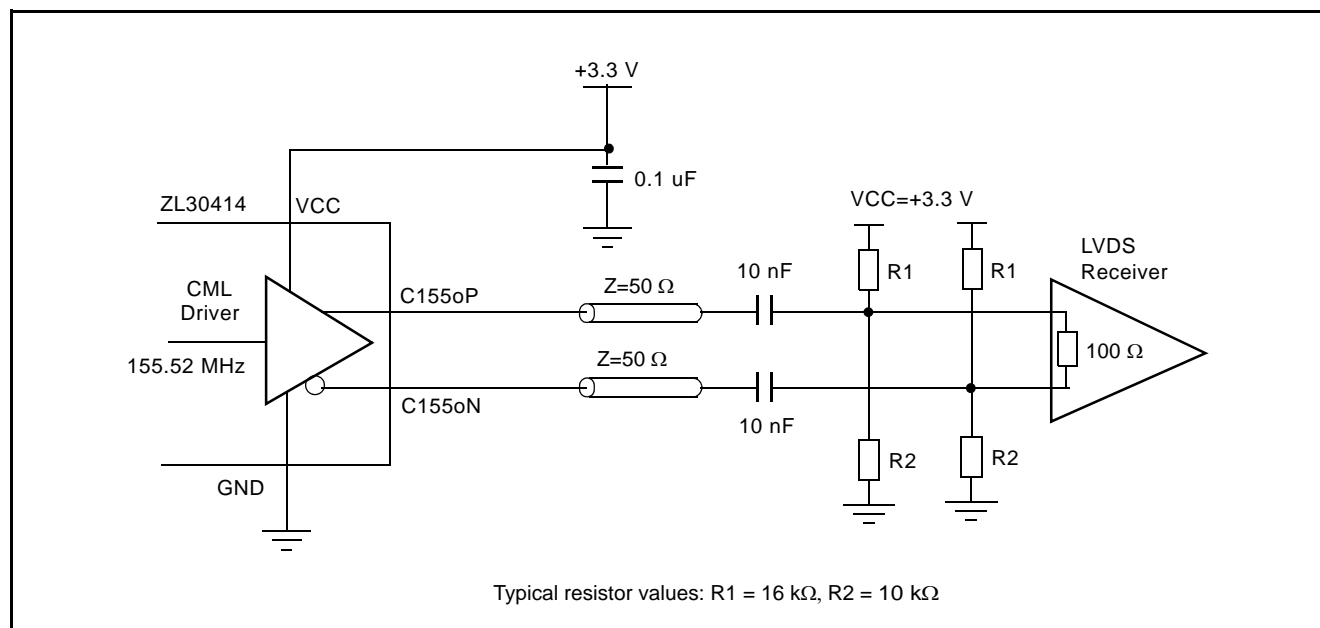
Figure 10 - LVDS Termination
