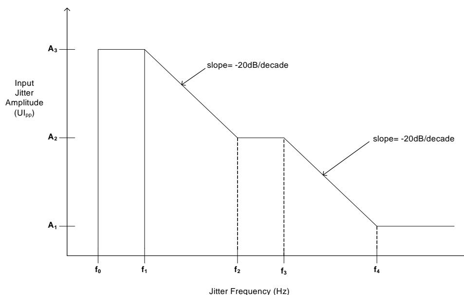
FIGURE 5. GR-253/G.783 JITTER TOLERANCE MASK
