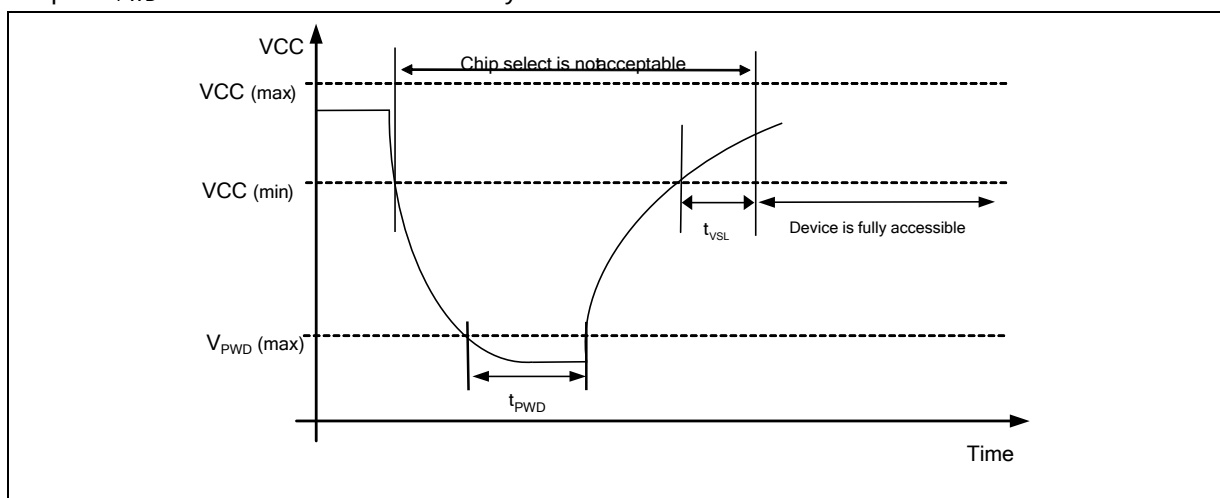
Figure 65c. Power Cycle Requirement
