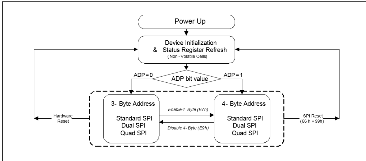
Figure 3. W25Q512JV Serial Flash Memory Operation Diagram
