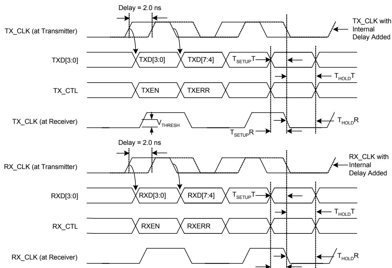
Figure 27. RGMII Compensated Timing
