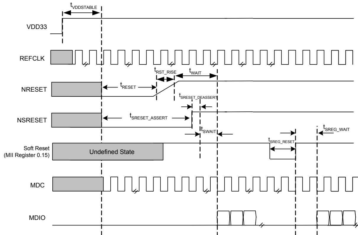
Figure 21. Reset Timing
