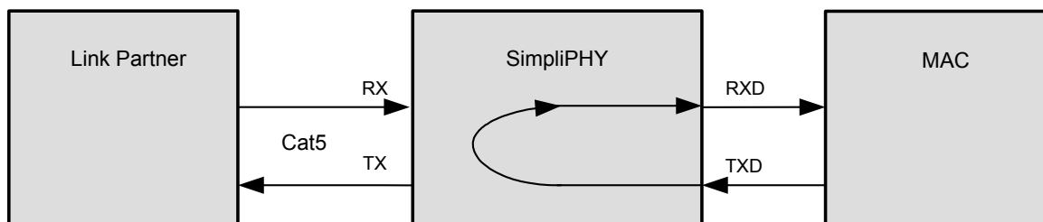
Figure 14. Near-End Loopback
