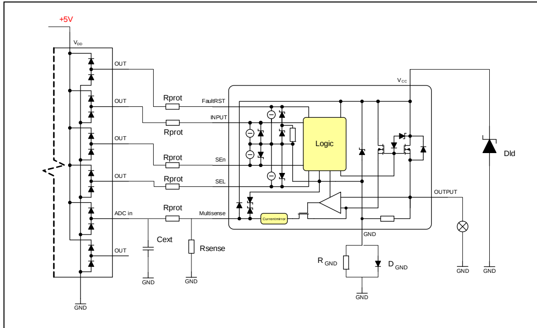
Figure 35. Application diagram
