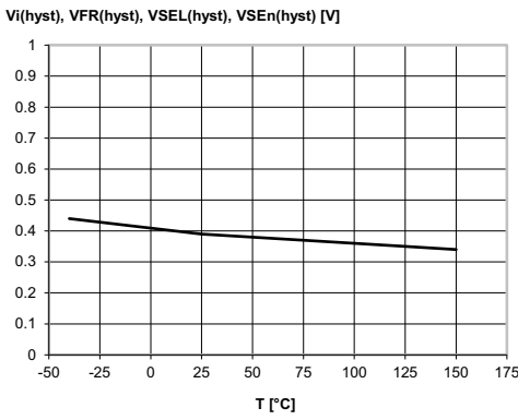
Figure 22. Logic Input hysteresis voltage
