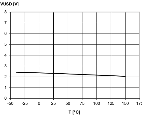
Figure 24. Undervoltage shutdown
