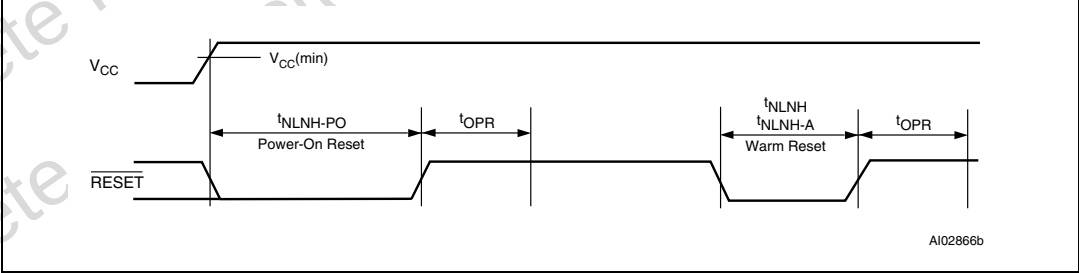
Figure 83. Reset (RESET) timing
