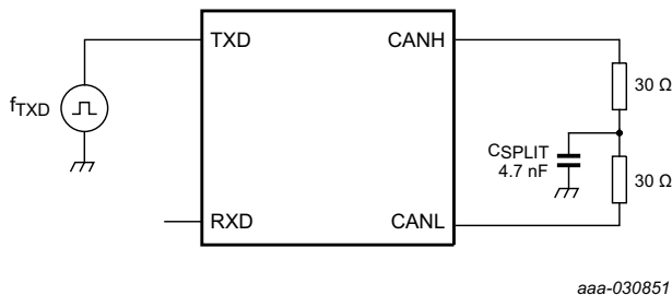
Fig 17. Test circuit for measuring transceiver driver symmetry
