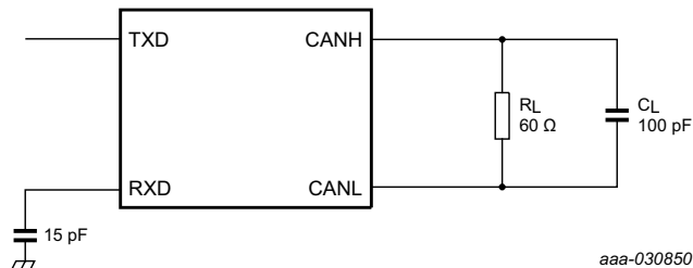
Fig 16. Timing test circuit for CAN transceiver
