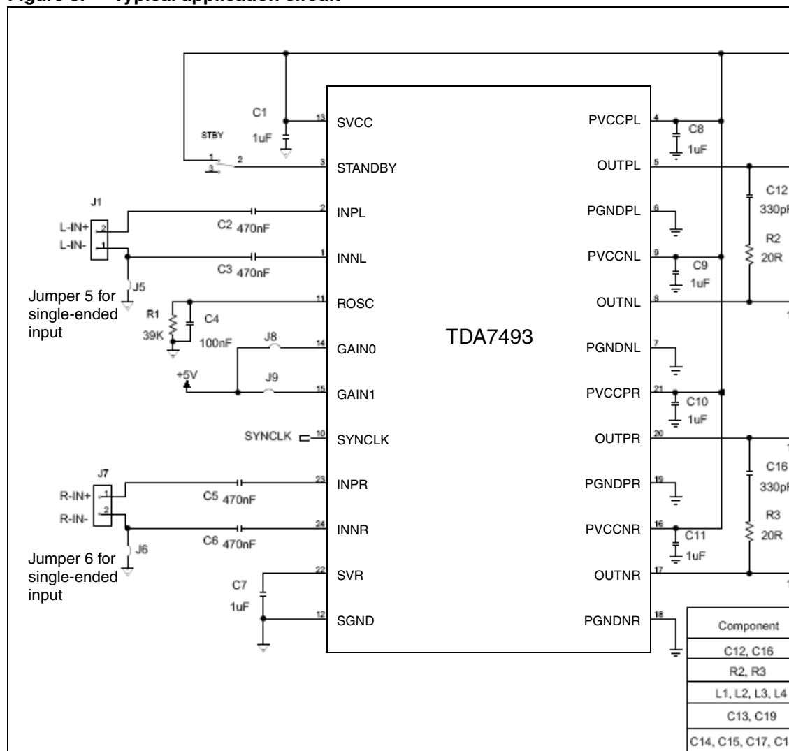
Figure 3. Typical application circuit
