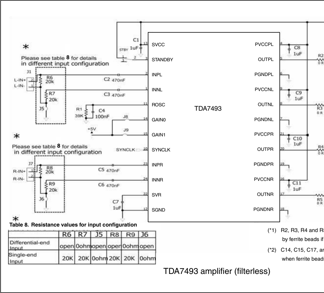
Figure 7. Schematic for the filterless configuration
