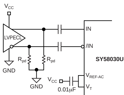
For a 3.3V system, R_{pd} = 100\Omega For a 2.5V system, R_{pd} = 50\Omega
