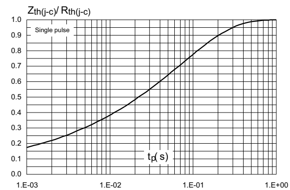
Figure 3. Relative variation of thermal impedance junction to case versus pulse duration (DPAK)
