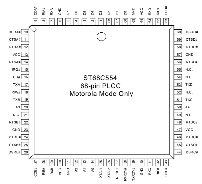
Figure 5: PLCC68 Pinout, Motorola Mode Only
