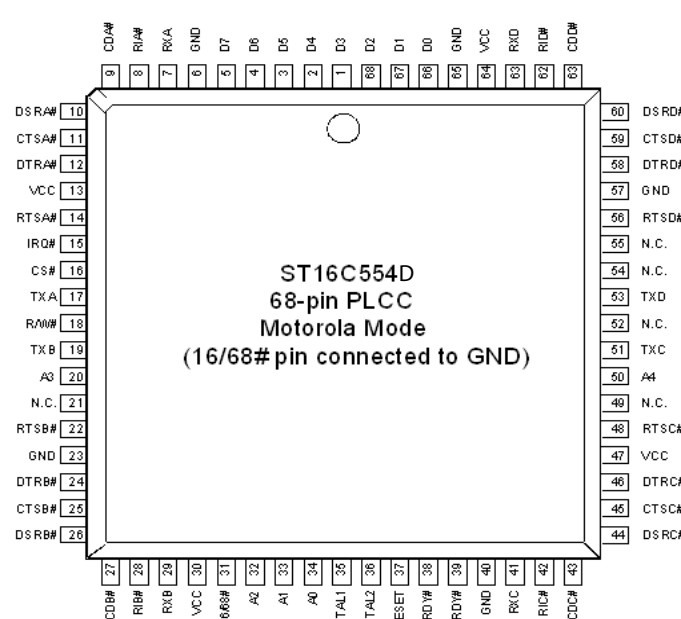
Figure 3: PLCC68 Pinout, Motorola Mode
