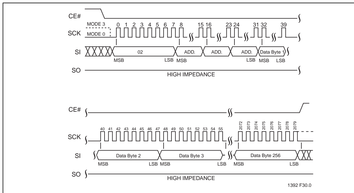
Figure 10: Page-Program Sequence
