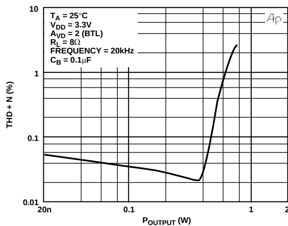
Figure 18. THD + N vs. P_{\text{OUTPUT}}
