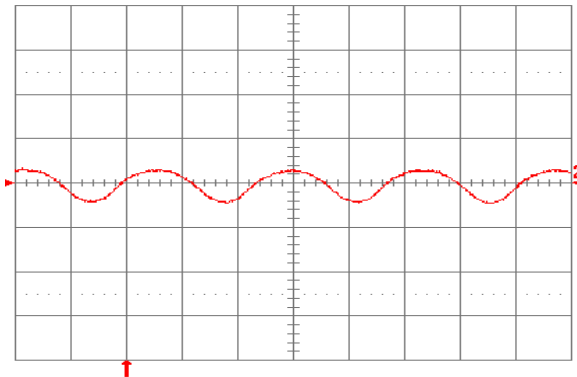
Fig. 1.5V.9: Input reflected ripple current, i_c (100 mA/div.), measured at input terminals at full rated load current and V_{in} = 48\ \text{V} . Refer to Fig. 1.5V.8 for test setup. Time scale: 1\ \mu\text{s}/\text{div} .
